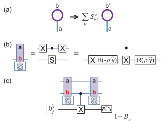
FIG. 10. (Color online) (a) S transformation acting on a two-qubit tadpole. The tensor S_{bb'} is defined in the text. (b) S circuit which carries out an S transformation. The 2 \times 2 matrix S is given in Eq. (9). Here, R(\pm\rho\hat{y}) = e^{\pm i\rho\sigma_y/2} are single-qubit rotations about the y axis with \rho = \tan^{-1}\phi^{-1} for which R(\rho\hat{y})XR(-\rho\hat{y}) = S . (c) Quantum circuit which uses the S circuit to measure B_p for a two-qubit tadpole.
